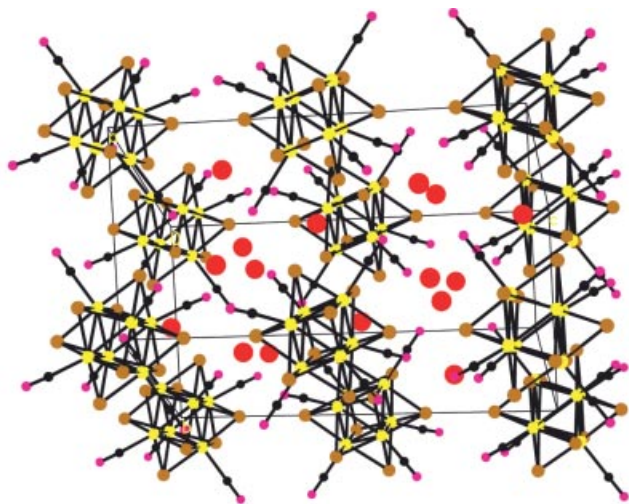
Figure 2. A view of the unit cell of \text{Cs}_5[\text{Mo}_6\text{Se}_{3.6}\text{Cl}_{4.4}(\text{CN})_6] ( 1 ); the yellow circles are Mo, the brown circles are Se/Cl, the black circles are C, the small red circles are N, and the large red circles are Cs atoms
